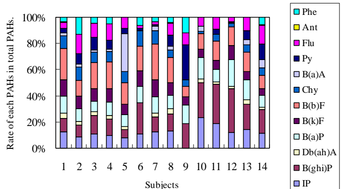
Fig. 4 Fractions of 12 PAHs in total PAHs.
