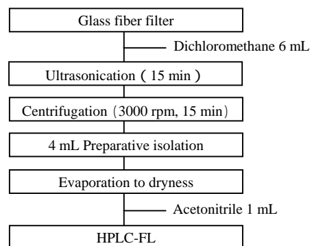
Fig. 2 Flow diagram for the filter sample preparation procedure.
